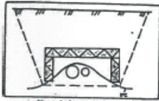
Hesteskoformet isolering.
